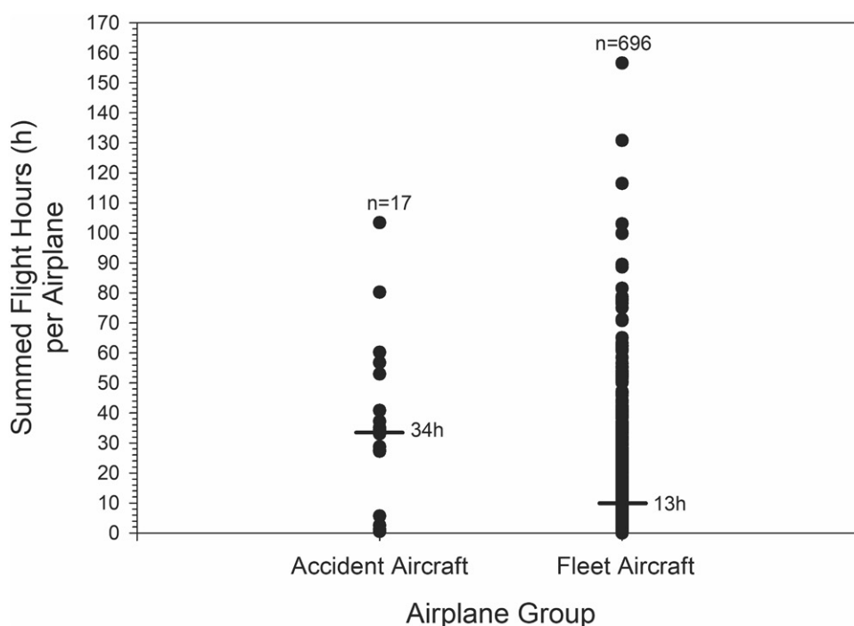
Fig. 4. Accident and fleet flight histories for a selected group of make/model airplane in specified U.S. states. Data shown are the ADS-B flight times summed for each aircraft (a filled circle representing a single airplane) in the specified group (accident and fleet) across the period spanning March–July 2020. The horizontal bars represent the median values for each population. The difference in the median values between the two groups was tested for significance using a Mann-Whitney U -test. n : airplane count.
