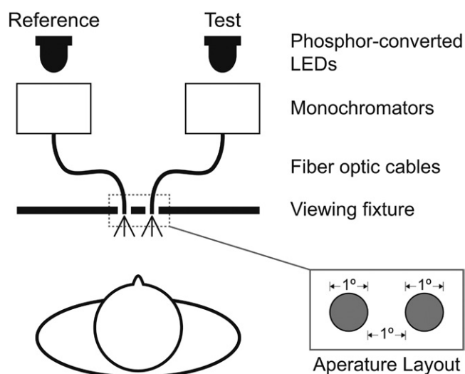
Fig. 1. Schematic diagram of the apparatus providing visual color stimuli for unique hue and wavelength discriminability measurements.
