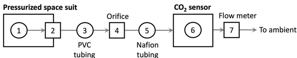
Fig. 2. Air sampling configuration. 1) Mouth guard sample probe; 2) suit pass-through port, open port potted with room temperature vulcanizing silicone; 3) 10-ft, 1/16-in ID Tygon® PVC tubing; 4) orifice sized to achieve 1000 ml · min -1 to sensor; 5) Nafion tubing; 6) infrared CO 2 sensor, AEI Technologies CD-3A; 7) flow meter for sample flow rate verification.
